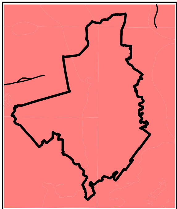
Solid Geology
