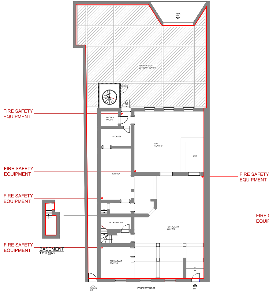
01 GROUND FLOOR PLAN 1:200 @A3
