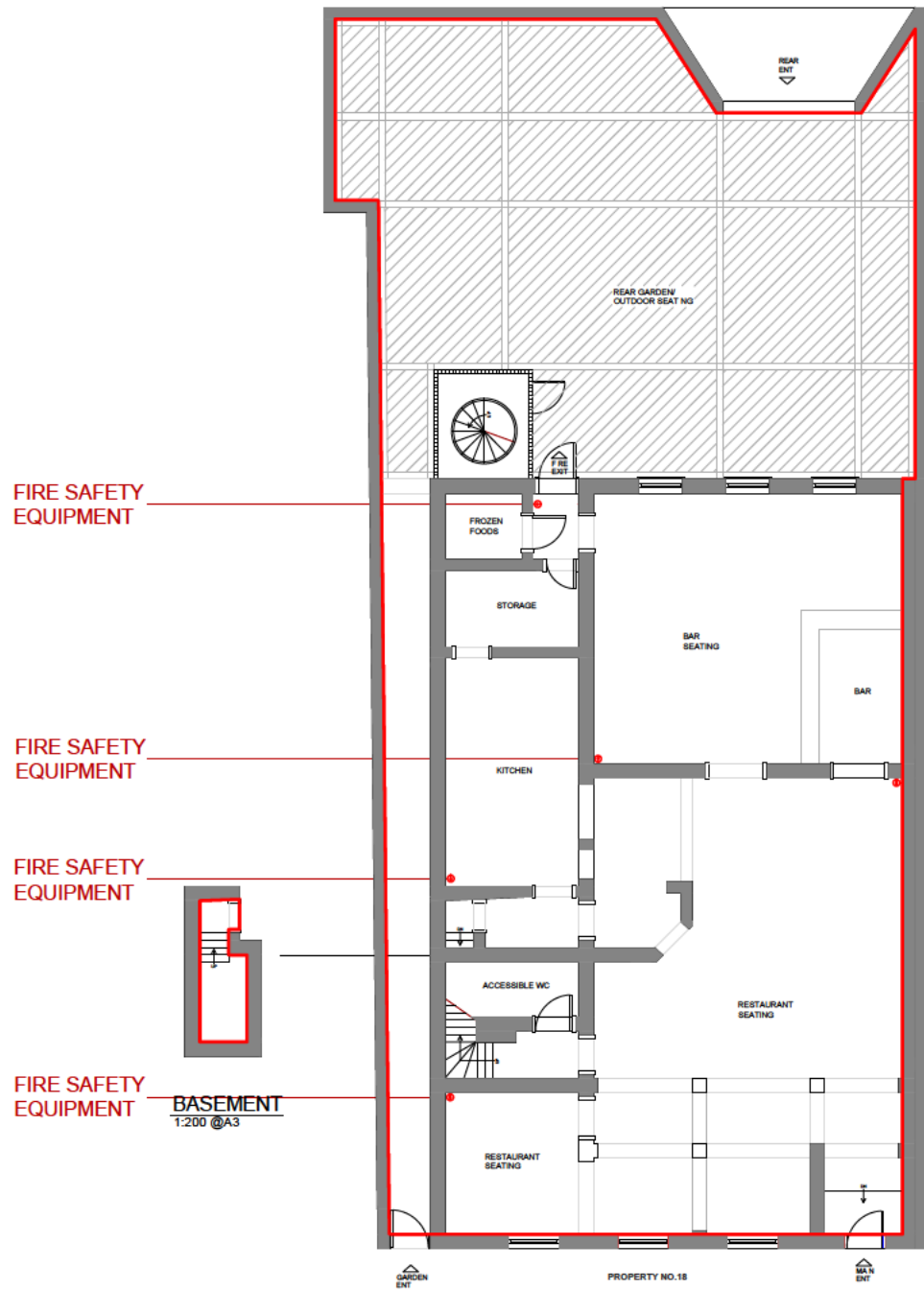
01 GROUND FLOOR PLAN 1:200 @A3
