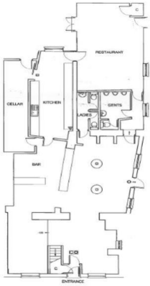
Ground floor Layout Plan 1:100
