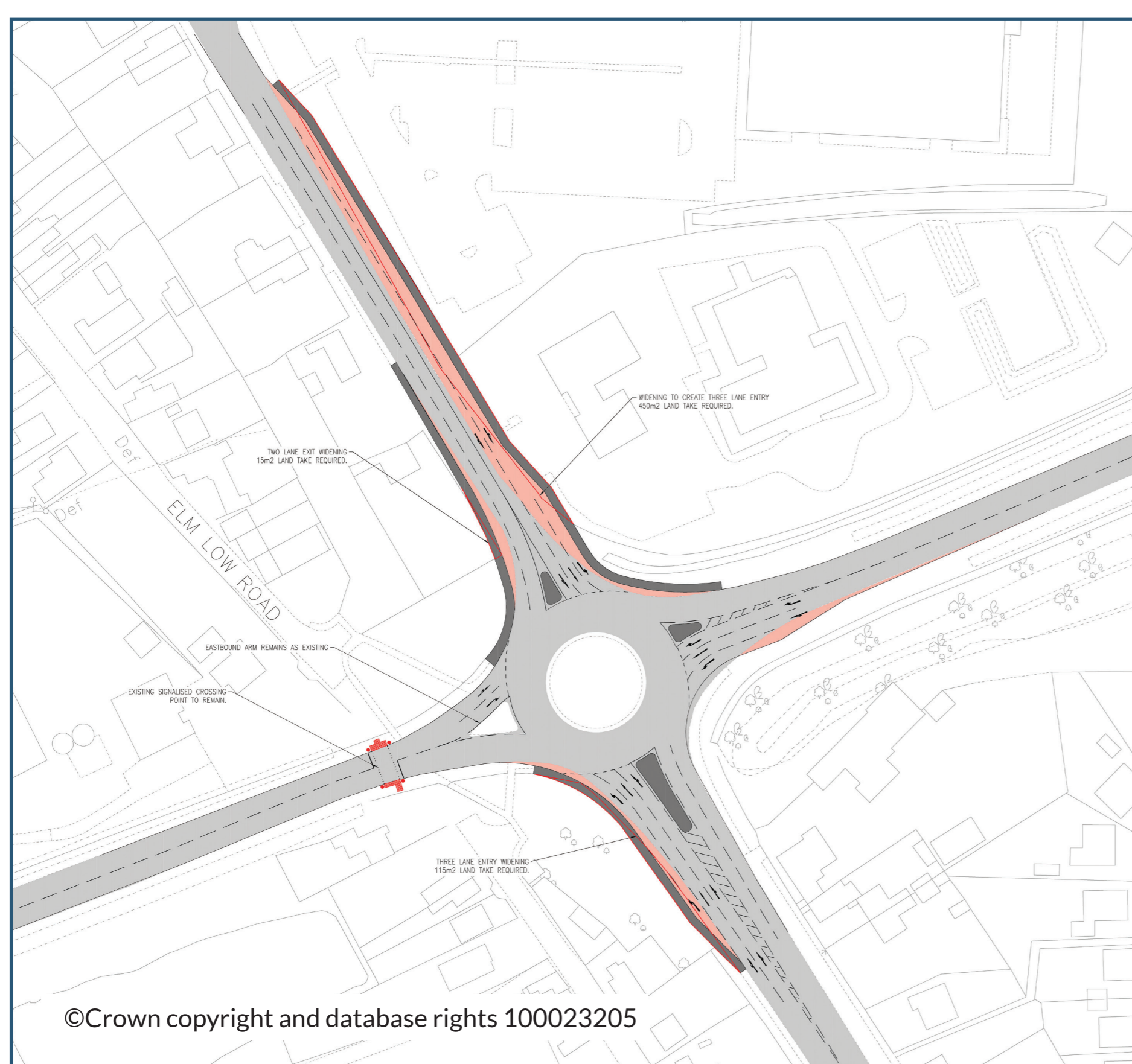
EH1 - Roundabout improvement in current location
