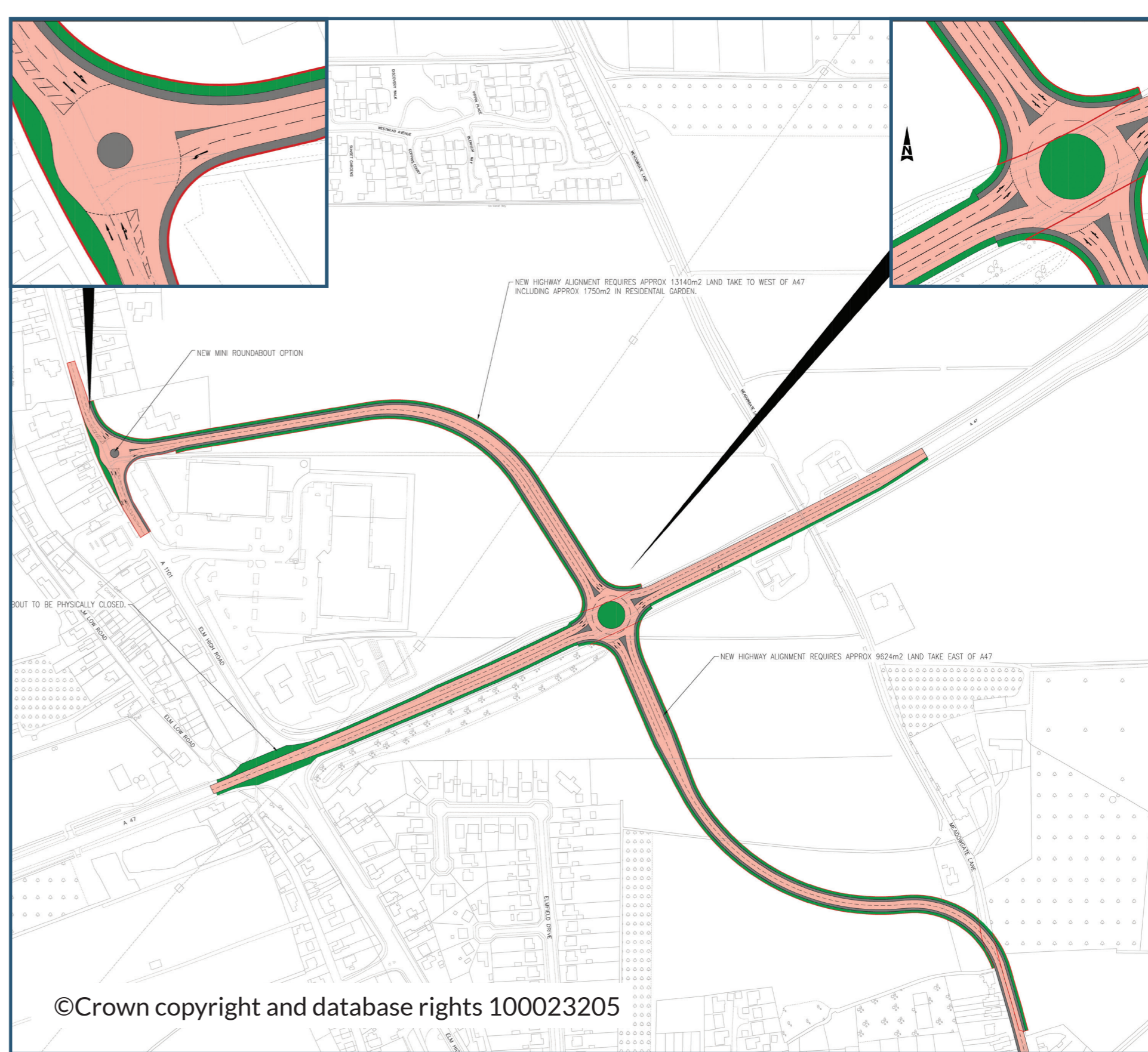
EH3B - Relocation of Roundabout further east
